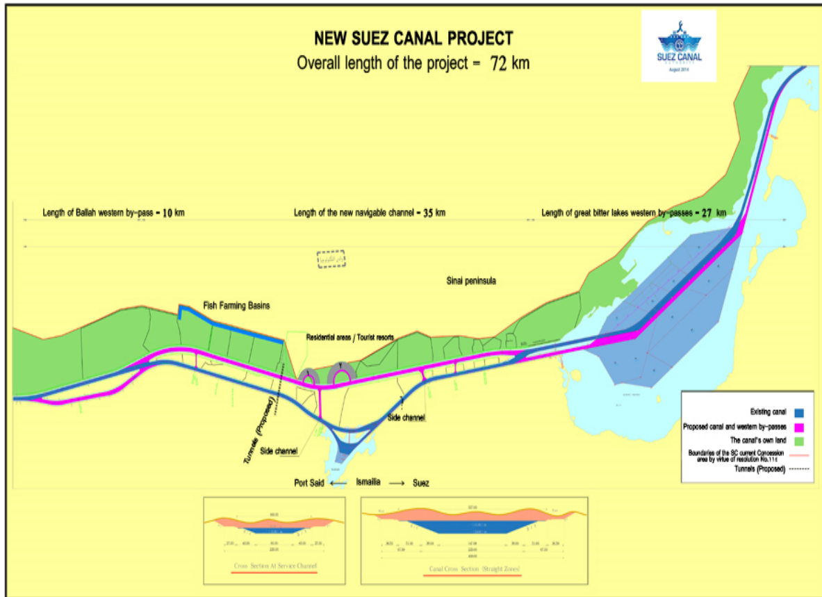
Figure (2) The new Suez channel design (14)
